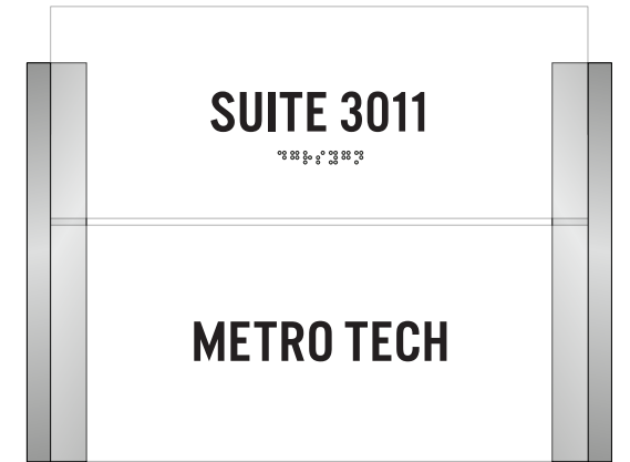
Configuration 56 Permanent Room ID, Multiple extended tile 11.0"w X 8.5"h
